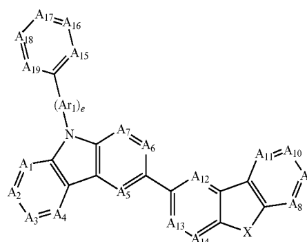
Chemical Formula 5
