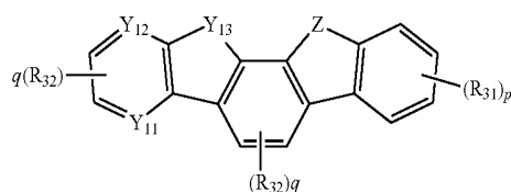
Chemical Formula 12
