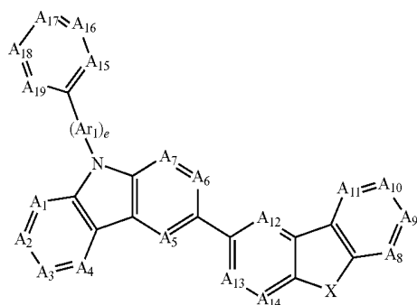
Chemical Formula 5
