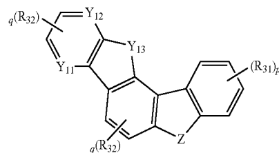
[Chemical Formula 13]
