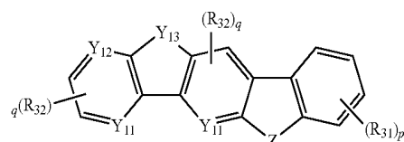
[Chemical Formula 12]
