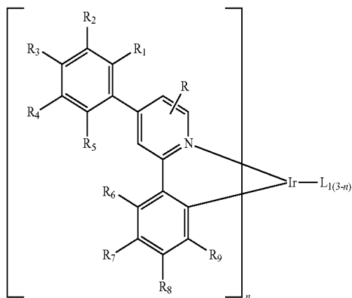
Chemical Formula 7
