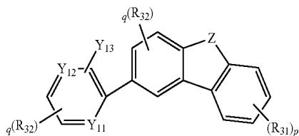
Chemical Formula 11
