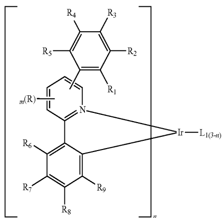
Chemical Formula 2
