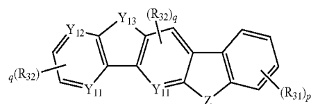
[Chemical Formula 12]
