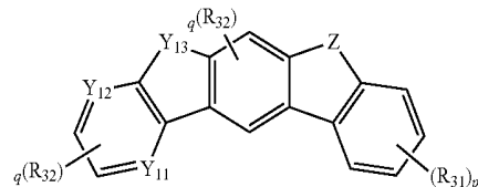
[Chemical Formula 11]
