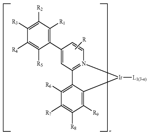
Chemical Formula 7
