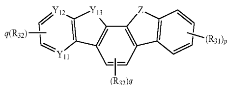
Chemical Formula 12
