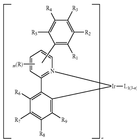
Chemical Formula 1
