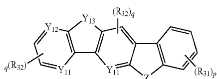
Chemical Formula 12
