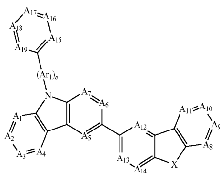
Chemical Formula 5
