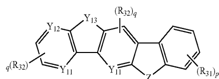
Chemical Formula 11
