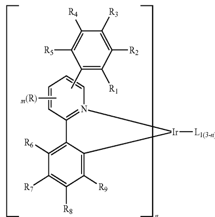
Chemical Formula 1
