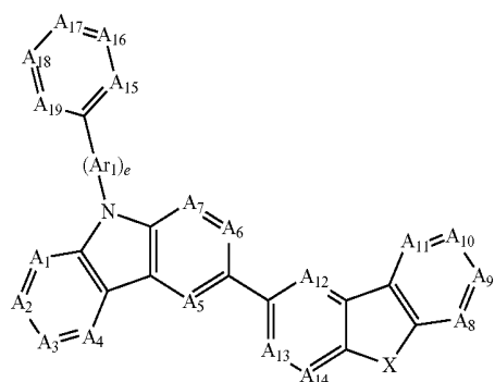
Chemical Formula 5
