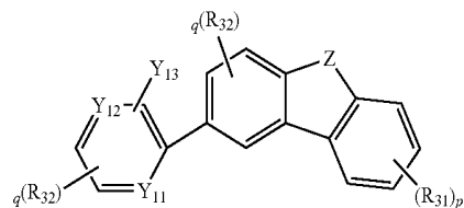
Chemical Formula 11
