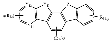
[Chemical Formula 13]
