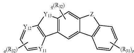
[Chemical Formula 11]
