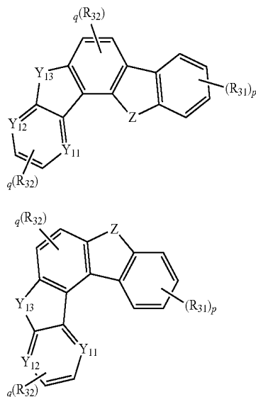
[Chemical Formula 9]
