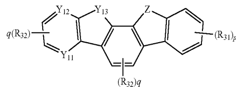
[Chemical Formula 13]
