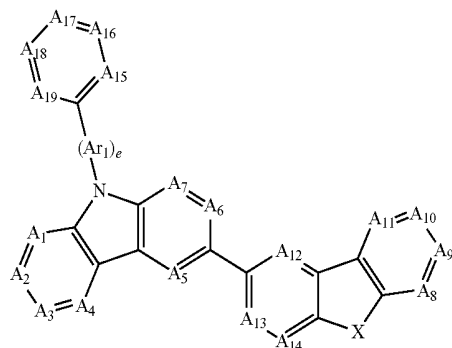
Chemical Formula 5
